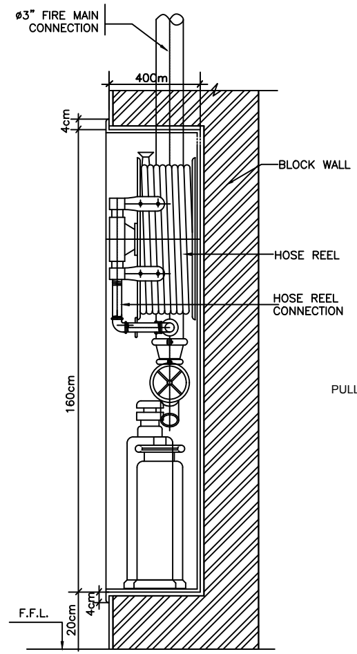
SECTIONAL SIDE ELEVATION
